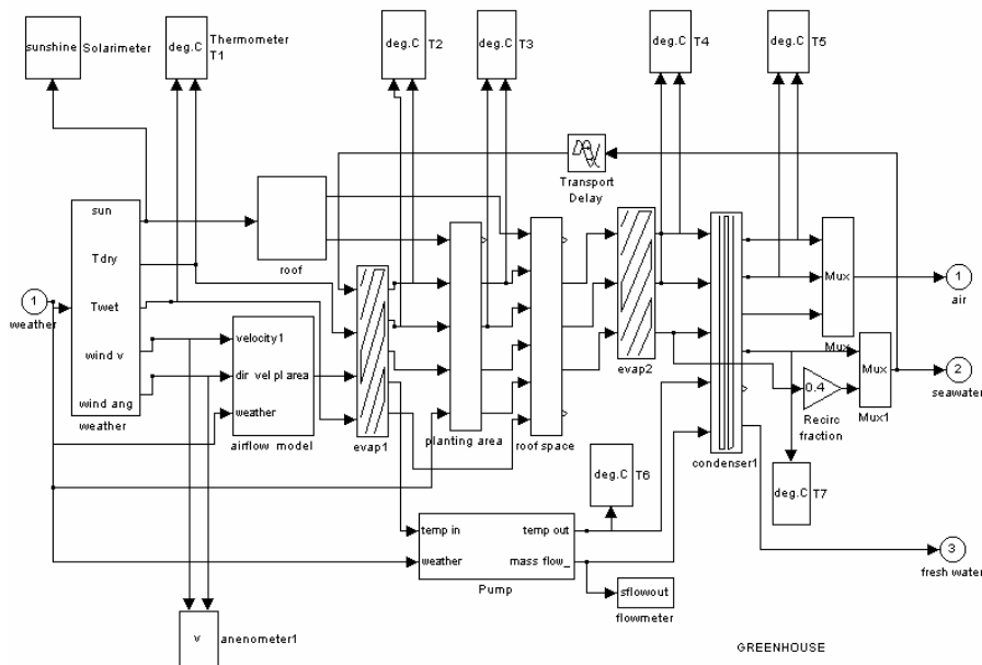
Figure 4: Overview of the thermodynamic model.
