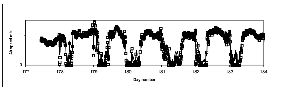
Figure 7: Verification of the wind driven airflow model against measurements of airspeed at the condenser of the Tenerife Greenhouse. The black line is predicted by the model and the square dots are measured values.
