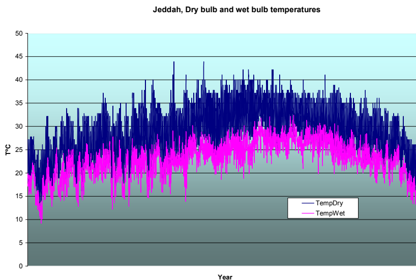
Figure 10 Comparison of average dry bulb and wet bulb temperatures throughout the year in Jeddah
